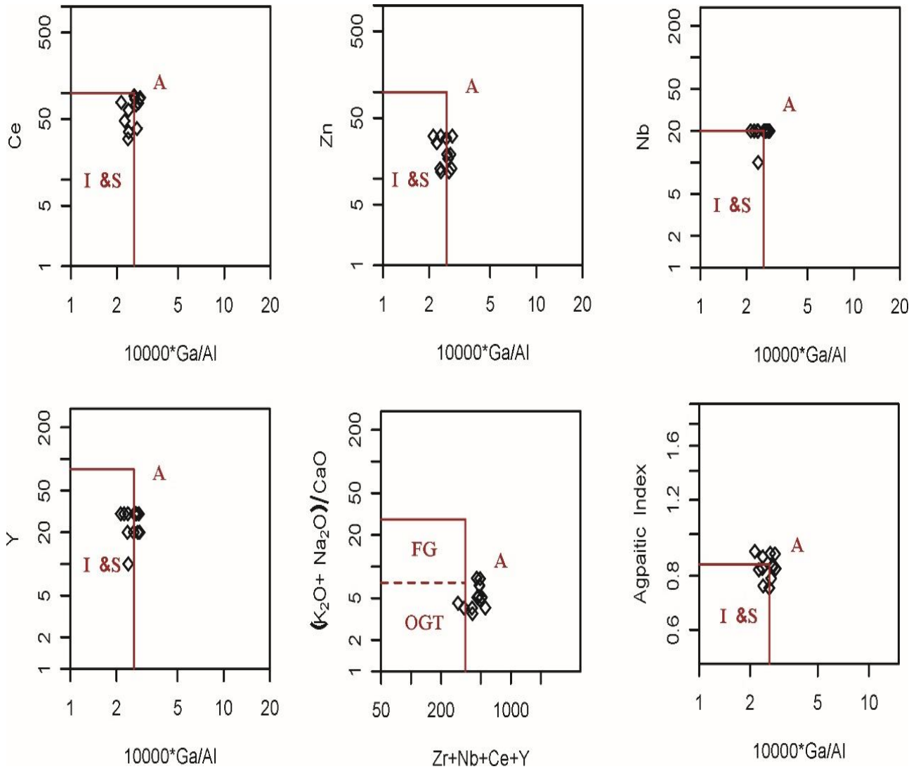
Fig. 17. Discrimination diagram between I-S and A-type granite (Whalen et al., 1987). The Takht granodiorite samples are plotted in border of A-type field.
