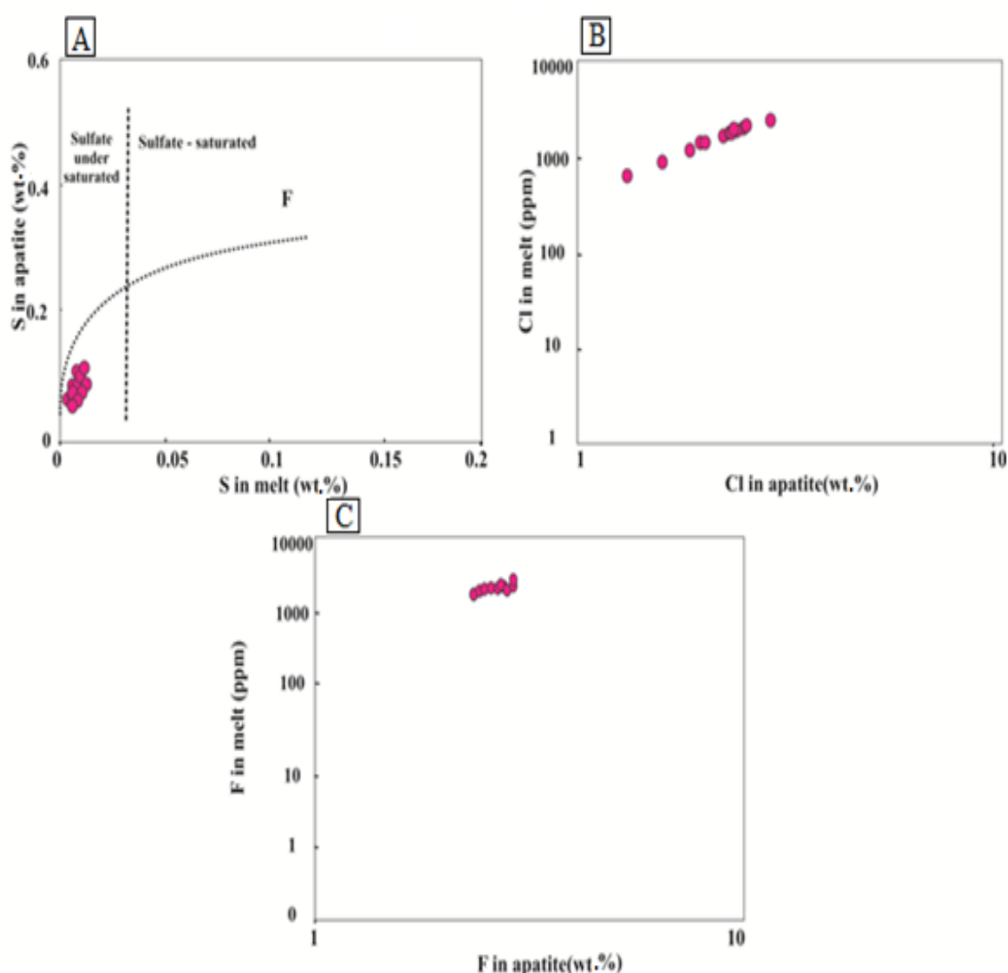
Fig. 7. Sulfur, Cl, and F concentrations in the melt and apatite in the Haftcheshmeh deposit: A: S in the melt (wt.%) vs. S in apatite (wt.%) diagram (Parat et al., 2011), B: the calculated Cl (ppm) content of the melt and Cl (wt.%) in the same apatite grains, and C: the calculated F (ppm) content of the melt and F (wt.%) in the same apatite grains. Abbreviations: Ap_m -magmatic apatite.
