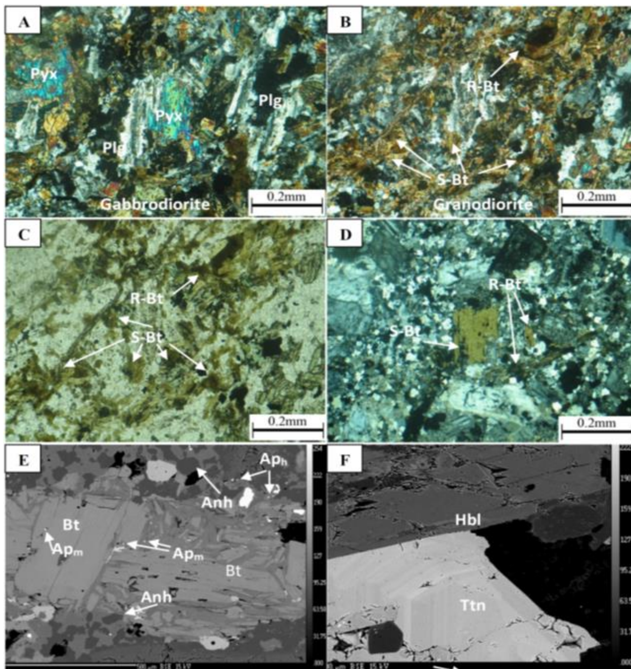
Fig. 4. Representative photomicrographs and back-scattered electron (BSE) images of biotite, amphibole, and apatite from gabbrodiorite and granodiorite porphyry of the Haftcheshmeh Cu-Mo porphyry system: A: Photomicrograph of gabbrodiorite with phenocrysts of plagioclase and pyroxene in ophitic texture (crossed polarized transmitted light), B: Reequilibrated biotite and secondary biotite in granodiorite porphyry associated with plagioclase (crossed polarized transmitted light), C: Reequilibrated biotite and secondary biotite associated with K-feldspar, quartz, and sericite in granodiorite porphyry (crossed polarized transmitted light), D: Photomicrograph of plagioclase phenocrysts replaced by hydrothermal biotite in granodiorite porphyry (crossed polarized transmitted light), E: Back-scattered electron (BSE) image of biotites and Ap grains partly as inclusions within biotite and anhydrite, and F: Back-scattered electron (BSE) image of hornblende and titanite. Abbreviations after Withney and Evans (2010) (BT: biotite, R-Bt: reequilibrated biotite, S-Bt, Secondary biotite, Plg: plagioclase, Pyx: Pyroxene, Ap h : hydrothermal apatite, Ap m : magmatic apatite, Ttn: Titanite, Anh: Anhydrite, hbl: Hornblende).
