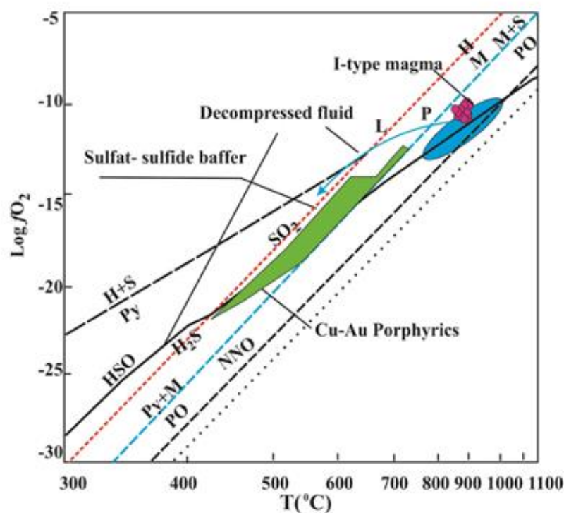
Fig. 6. Compositions of apatites from the Haftcheshmeh deposit on Oxygen T(°C) vs. log fO_2 diagram for the oxygen fugacities of oxidized porphyry deposits (Sun et al., 2015); Abbreviations: MH-Magnetite-Hematite buffer curve; NNO-Nickel-Nickel Oxide buffer curve; FMQ-Fayalite-Magnetite-Quartz buffer curve.
