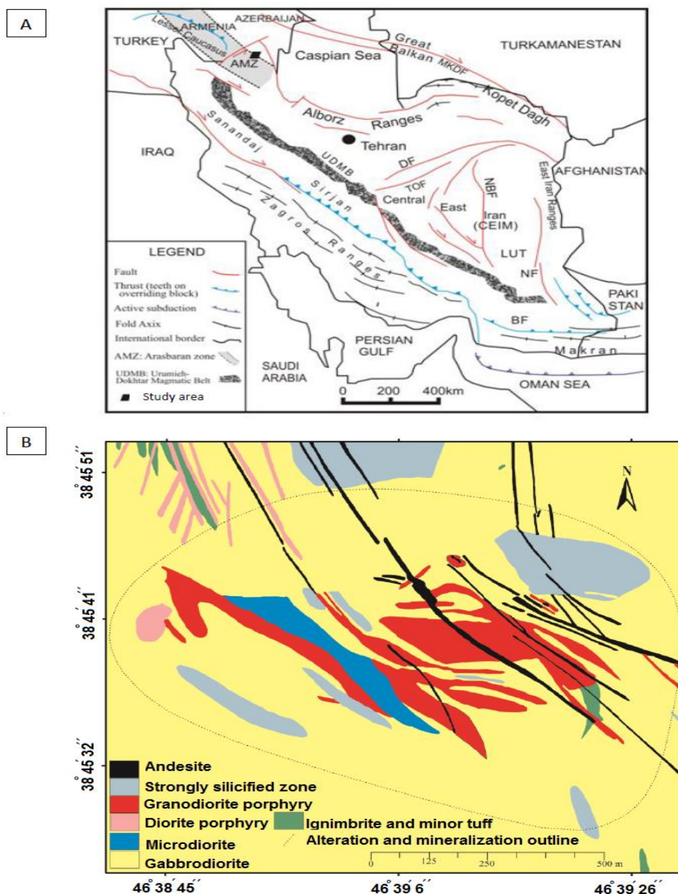
Fig. 1. A: Simplified geology map of Iran (modified from Nabavi, 1976), showing the Haftcheshmeh Cu-Mo porphyry in the Alborz-Azarbaijan structure zone, NW Iran, and B: Geological map of the Haftcheshmeh ore deposit (Hassanpour and Moazzen, 2018)
