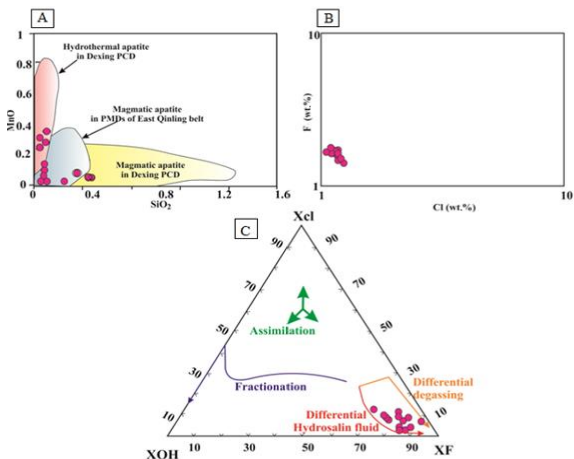
Fig. 5. Major and trace element compositions in Ap from the Haftcheshmeh porphyry deposit: A: Plot of SiO 2 vs. MnO for apatites hosted in gabbrodiorite and granodiorite porphyry. The fields of magmatic and hydrothermal apatite in Dexing porphyry Cu deposit (PCD) and porphyry Mo deposits (PMDs) of East Qinling belt are from Zhao et al. (2020), B: Cl vs. F, and C: Ternary F-Cl-OH diagram McCubbin et al. (2015). The XF-XCl-XOH are the mole fractions of each volatile component, as defined in Table 1.
