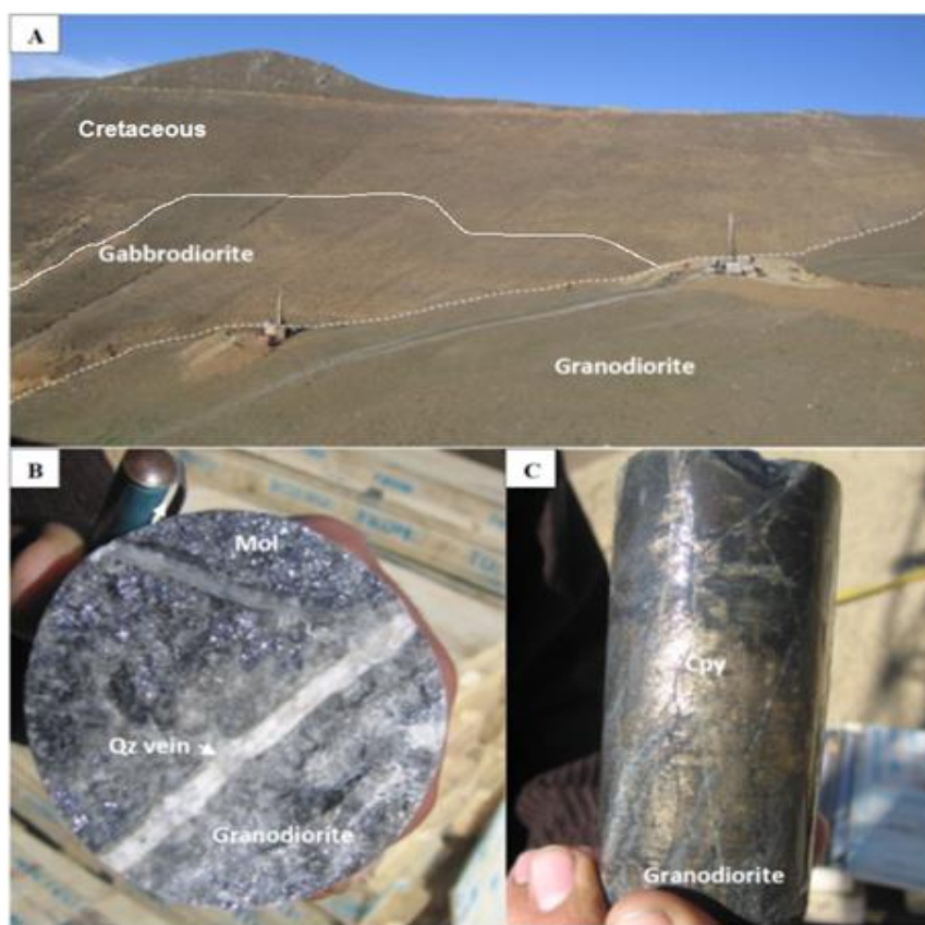
Fig. 2. Representative photographs of the field and drill cores from the Haftcheshmeh Cu-Mo porphyry system: A: Outcrop of the gabbrodiorite and granodiorite porphyry intrusions in the Haftcheshmeh area (NE landscape), B: Molybdenite and D type quartz veinlets in the granodiorite porphyry stock, and C: Chalcopyrite and pyrite mineralizations in the granodiorite porphyry stock. Abbreviations after Withney and Evans (2010) (Mol: Molybdenite, Qz: Quartz).
