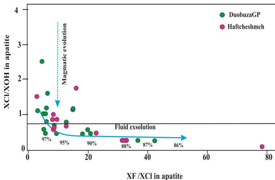
Fig. 8. Comparison of changes in volatile apatite elements from the porphyry of Haftcheshmeh with changes in apatite volatile elements from intrusions of Duolong porphyry Cu-Au deposit. These figures show compositional changes in volatile apatite elements during the evolution from volatile-undersaturated to volatile-saturated magma. XF/XCl vs. XCl/XOH in apatite; Blue solid curves in diagram calculated by the Rayleigh fractionation model represent the variation of volatile elements in apatite during fluid exsolution. Data from apatite inclusions in biotite phenocrysts from ore-bearing granodiorite porphyries of Duolong porphyry Cu-Au deposit are from Li et al. (2020) . Abbreviations: GP: granodiorite porphyry.
