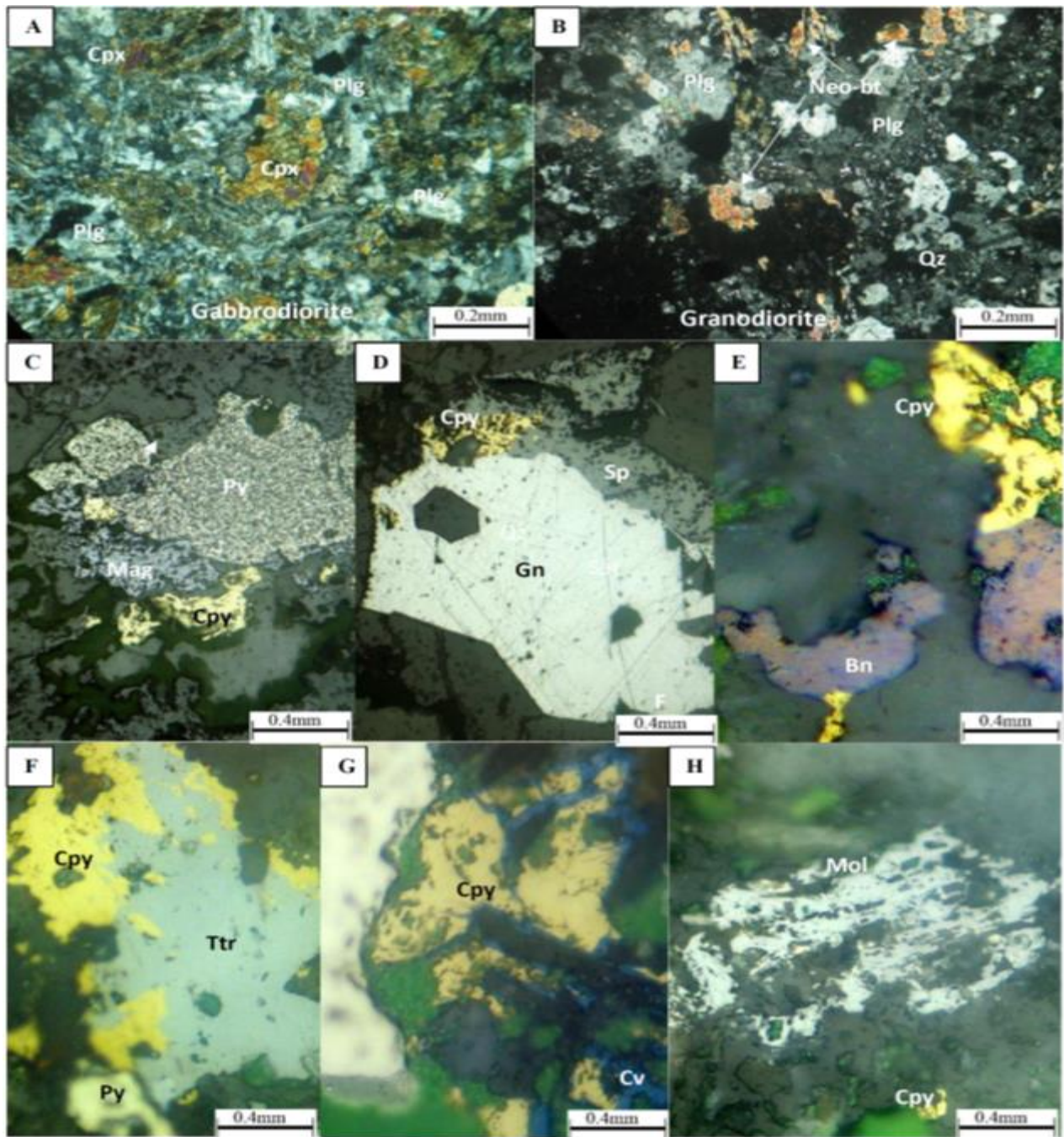
Fig. 3. Petrology and mineralogy of the Haftcheshmeh deposit: A: Phenocrysts of the plagioclase and pyroxene in an ophitic texture from fresh gabbrodiorite stock (crossed polarized transmitted light), B: Phenocrysts of plagioclase, quartz, ferromagnesian (Biotite and hornblende) and opaque minerals in a granodiorite porphyry texture, C: chalcopyrite-pyrite and magnetite in granodiorite porphyry from potassic alteration zone, D: chalcopyrite, galena and sphalerite in the sample from the propylitic alteration zone, E: bornite, and chalcopyrite from potassic alteration zone in gabbrodiorite, F: chalcopyrite, pyrite, and tetrahedrite in the potassic alteration zone, G: replacement of chalcopyrite by covellite minerals in the potassic alteration zone, and H: Molybdenite and chalcopyrite in the potassic alteration zone in Haftcheshmeh porphyry system. Abbreviations after Withney and Evans (2010) (Mol: Molybdenite, Cpx: Clino-Pyroxene, Plg: plagioclase, Bt: biotite, Gn: Galeana, Sp: Sphalerite, Py: pyrite, Cpy: chalcopyrite, Cv: covellite, Ttr: tetrahedrite, Bn: bornite, Mag: Magnetite).
