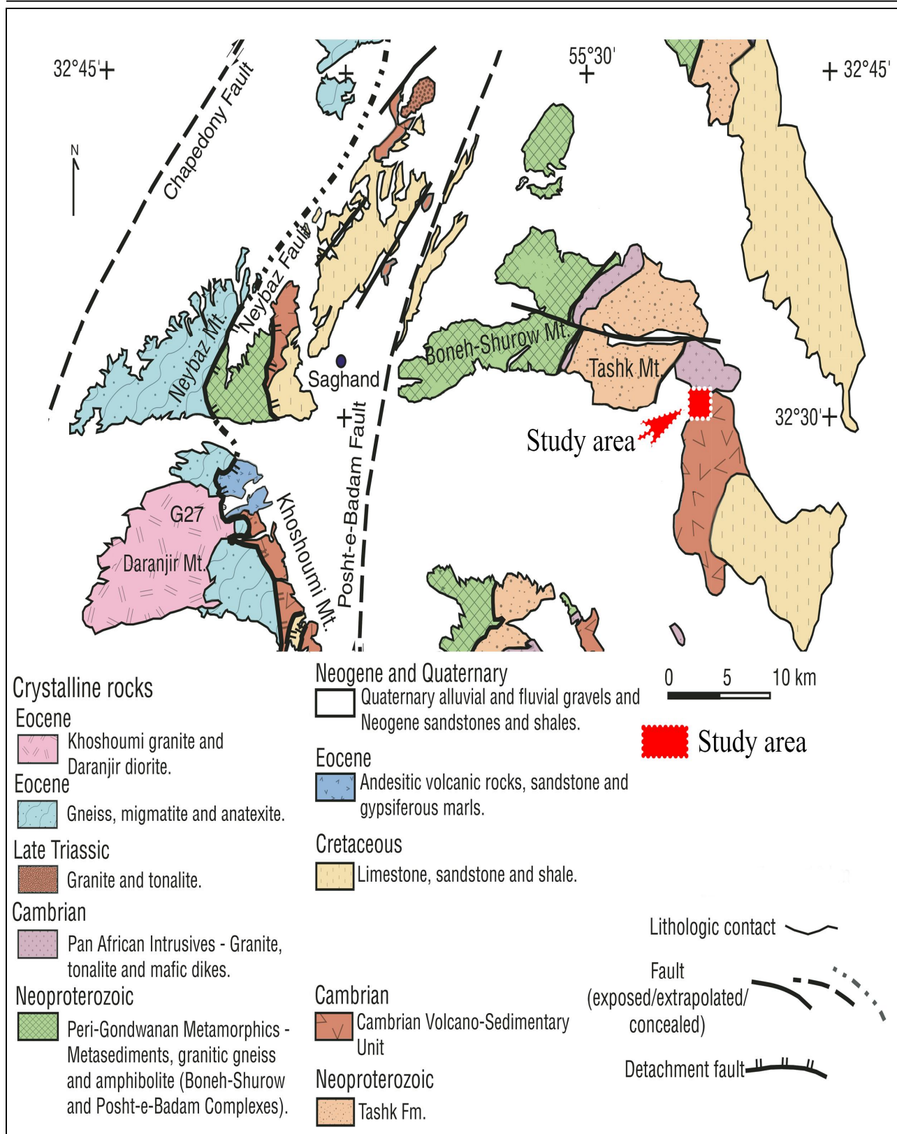
Fig. 2. Geologic map of the Saghand area (Verdel et al., 2007), Coordinate framework of this map is shown as red box on the Fig. 1.
