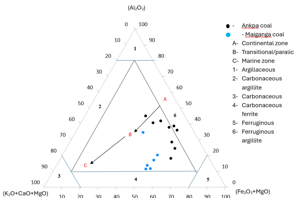
Fig. 11. \text{Al}_2\text{O}_3 - (\text{K}_2\text{O}+\text{CaO}+\text{MgO}) - (\text{Fe}_2\text{O}_3+\text{MgO}) [AKF] Ternary plot of Ankpa and Maiganga coal samples. Samples were deposited within continental and paralic depositional environment
